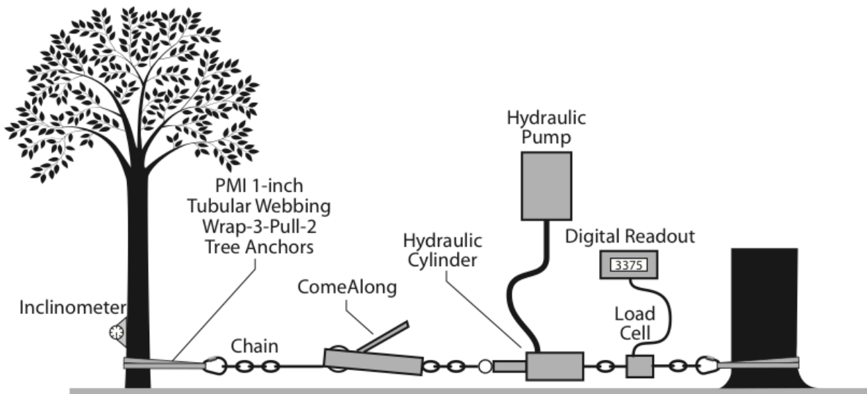
Figure 1 – Testing Rig.
